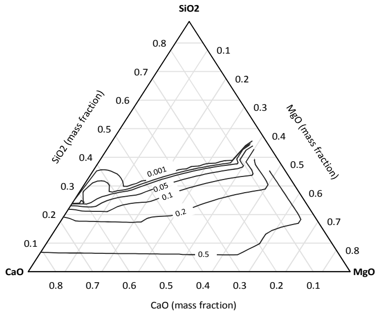
Figure 7: Volume fraction of solids ternary diagram of the SiO 2 -CaO-MgO-Al 2 O 3 system, with 12.5% Al 2 O 3
