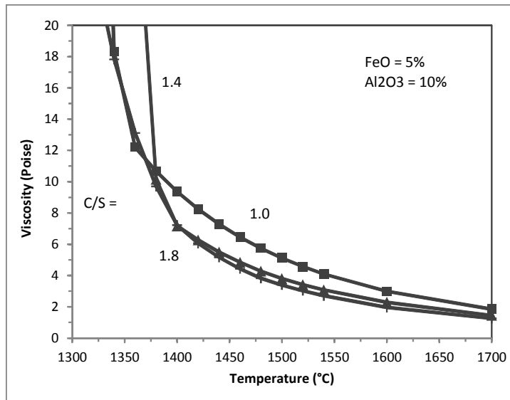
Figure 13: Effective viscosity as a function of temperature for FeO = 5%, Al 2 O 3 = 10%, and C/S = 1, 1.4, and 1.8
