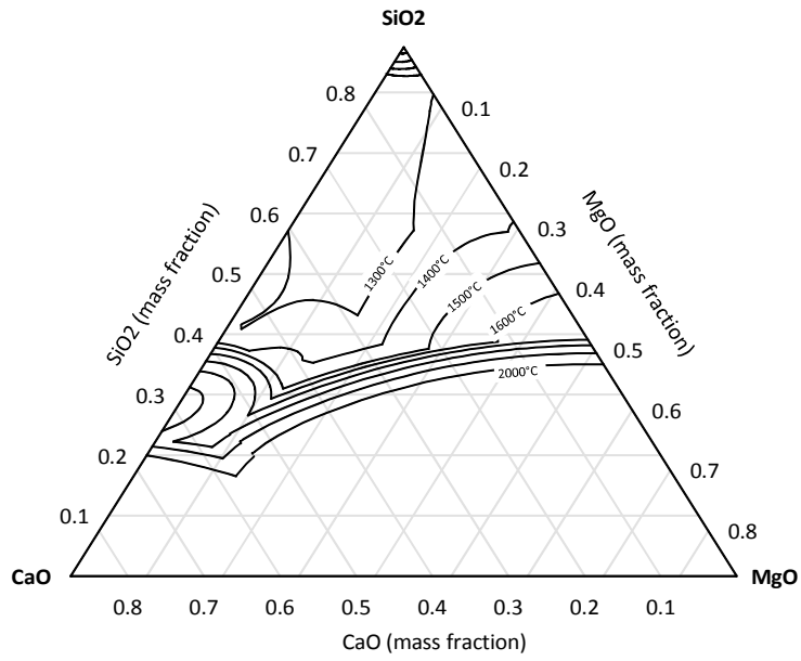
Figure 5: Liquidus temperature ternary diagram of the \text{SiO}_2\text{-CaO-MgO-Al}_2\text{O}_3 system, with 12.5% \text{Al}_2\text{O}_3
