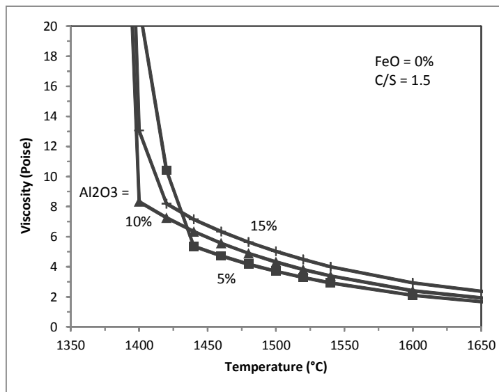
Figure 10: Effective viscosity as a function of temperature for \text{FeO} = 0\% , \text{C}/\text{S} = 1.5 , and \text{Al}_2\text{O}_3 = 5\% , 10\% , and 15\%
