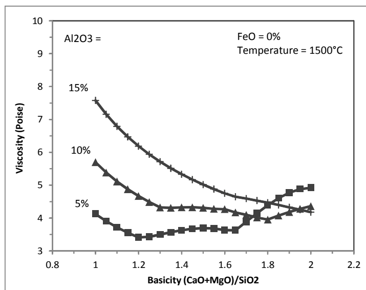
Figure 8: Effective viscosity as a function of basicity ((\text{CaO}+\text{MgO})/\text{SiO}_2) at 1500°C for FeO = 0%, and Al 2 O 3 = 5%, 10%, and 15%
