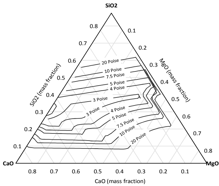
Figure 6: Effective viscosity ternary diagram of the \text{SiO}_2\text{-CaO-MgO-Al}_2\text{O}_3 system, with 12.5% \text{Al}_2\text{O}_3
