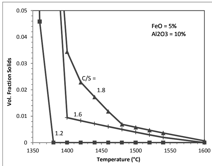
Figure 14: Volume fraction of solids as a function of temperature for FeO = 5%, Al 2 O 3 = 10%, and C/S = 1.2, 1.4, and 1.8
