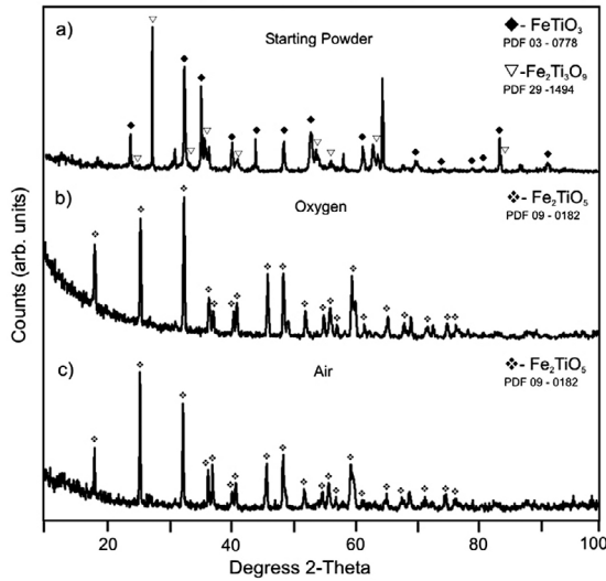
Figure 5: XRD patterns of NIC before and after milling for 10 minutes using EDAMM in oxidising atmospheres where (a) is the NIC starting powder, (b) milled in O_2 gas and (c) milled in air
