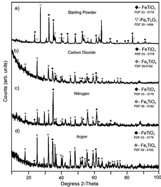
Figure 2: XRD patterns of NIC before and after milling for 10 minutes using EDAMM in various atmospheres where (a) is the NIC starting powder, (b) milled in \text{CO}_2 gas, (c) milled in \text{N}_2 gas and (d) Milled in Ar gas
