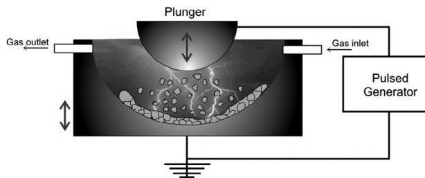
Figure 1: A schematic of the Electric Discharge Assisted Mechanical Milling (EDAMM) technique
