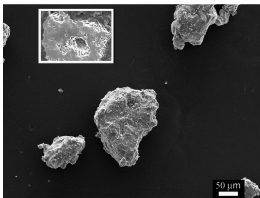
Figure 6: SEM secondary electron image showing the ilmenite sample after reaction in EDAMM for 10 minutes in air. Inset shows cross sectioned particle image. The scale bar is 50 \mu\text{m}
