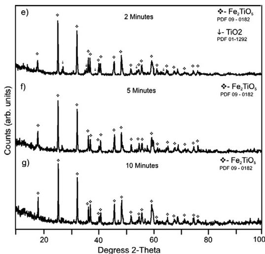
Figure 8: XRD patterns of NIC before and after EDAMM processing for times up to 10 minutes in an air atmosphere
