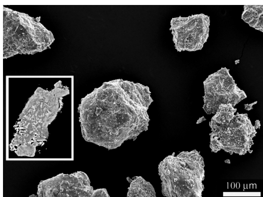
Figure 4: SEM secondary electron image showing the NIC sample after reaction in EDAMM for 10 minutes under Ar gas. The scale bar is 100 μm
