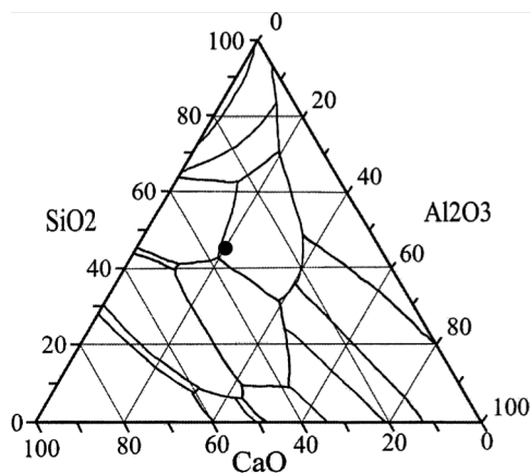
Figure 1: CAS ( \text{CaO-Al}_2\text{O}_3\text{-SiO}_2 ) ternary phase diagram
