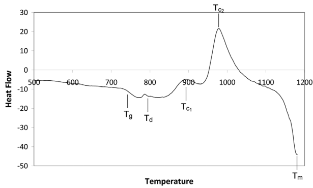
Figure 2: DTA heat curve for the vitreous sample
