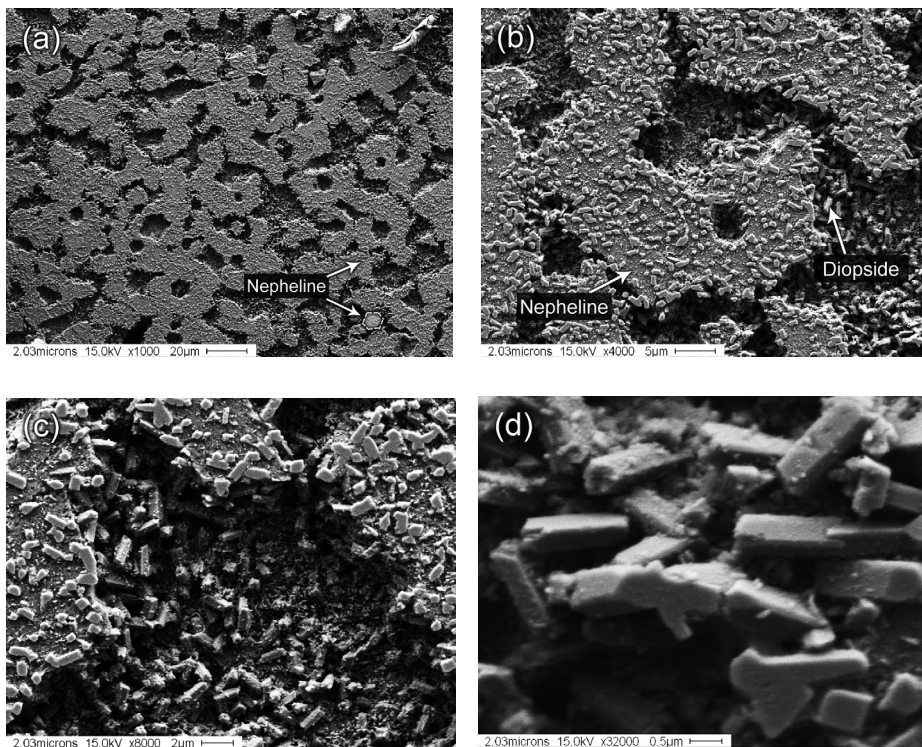
Figure 6: SEM micrographs of the produced glass-ceramic material at different magnifications showing crystals of hexagonal Nepheline and monoclinic Diopside: (a) x1000, (b) x4000, (c) x8000, and (d) x32000
