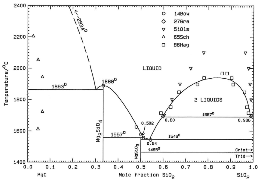
Fig. 1: Optimized MgO-SiO 2 phase diagram.
